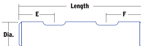
STYLE 9: DUAL KEYWAY
