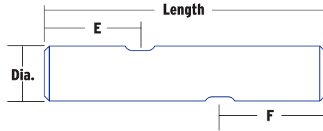
STYLE 2: TWO KEYWAYS
