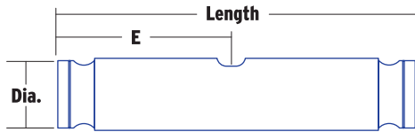
STYLE 3: ONE KEYWAY, TWO SEAL GROOVES
